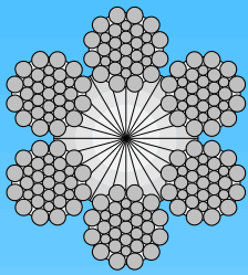
6x31WS-SFC Warrington-Seale
