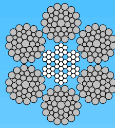
6x36WS-IWRC Warrington-Seale
