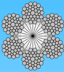
6x36WS-SFC Warrington-Seale
