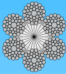
6x41WS-SFC Warrington-Seale
