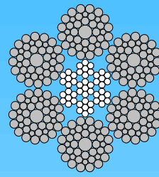
6x41WS-IWRC Warrington-Seale
