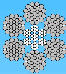
6x31WS-IWRC Warrington-Seale
