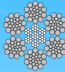
6x26WS-IWRC Warrington-Seale
