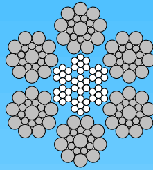
6x19S-IWRC Seale
