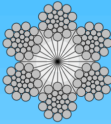
6x26WS-SFC Warrington-Seale
