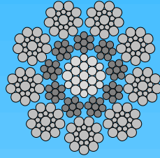
9x19S-PWRC Seale
