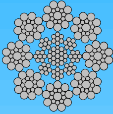
8x19S-IWRC Seale
