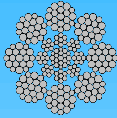
8x19W-IWRC Warrington
