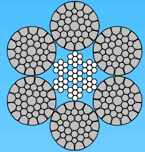
6xK36WS-IWRC Warrington-Seale
