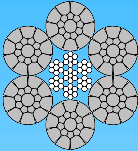
6xK19S-IWRC Seale
