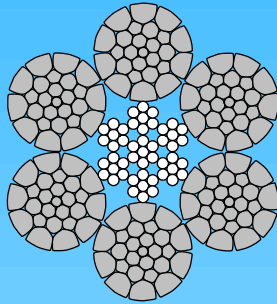
6xK26WS-IWRC Warrington-Seale
