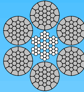
6xK31WS-IWRC Warrington-Seale
