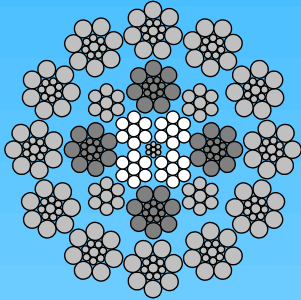
24(W)x7 Rotex-Ultra 12x19S-12(W)
