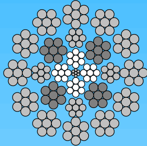
24(W)x7 Rotex-Ultra 12x7-12(W)
