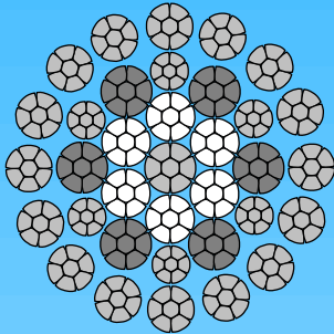
35(W)xK7 Rotex-Plus MasterForm™
